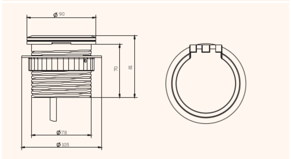
Technical Drawing
